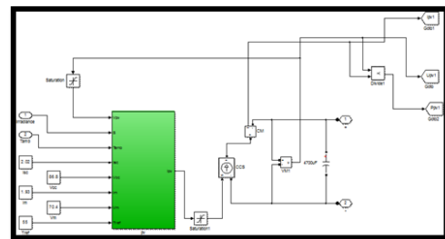
Fig. 3: PV Matlab / Simulink Model.
