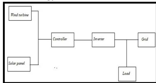
Fig. 2: Block Diagram of Hybrid Energy System.
