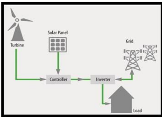
Fig. 1 Hybrid Energy System.
