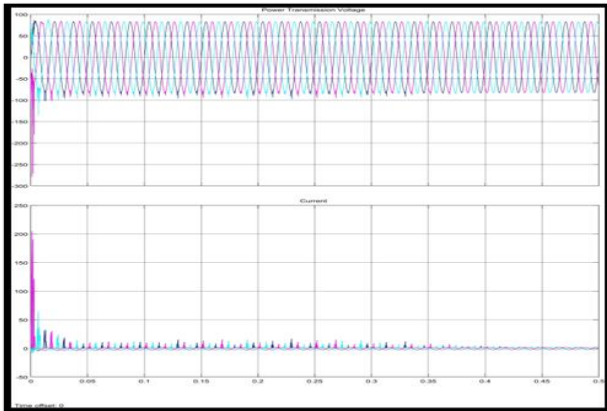
Fig. 5: Simulation Result of output of Hybrid Energy System.
