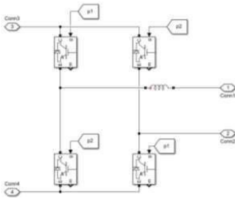
Figure.5. Simulation of Single-Phase Inverter
