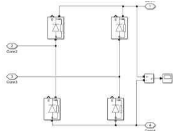
Figure.3. Uncontrolled rectifier
