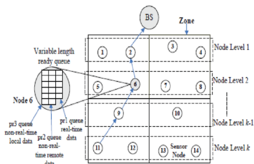
Fig.2 Proposed dynamic multilevel priority (DMP) packet scheduling scheme
