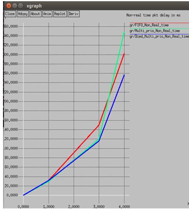
Fig.8 Non-real time packet delay
