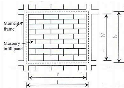
Figure: Masonry infill panel in frame structure Infill wall without opening
