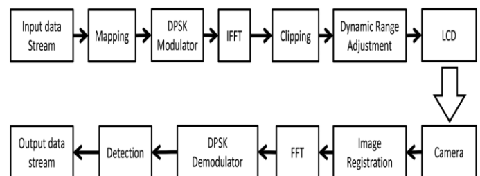
Fig.: Basic block diagram for data transfer using QR codes from one phone to another
