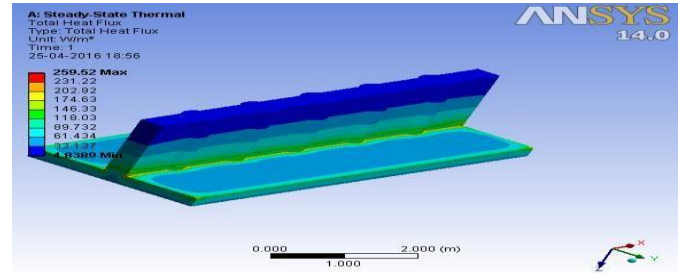
Total heat flux for circular extension fin
